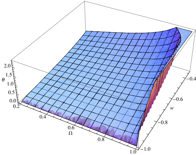
Figure 5. Three-dimensional plot of \theta_{\text{DE}}(z = 2.80) as a function of (\Omega_\phi, w_\phi) in the range \Omega_\phi = [0.2, 1] and w_\phi = [-0.34, -1] .
