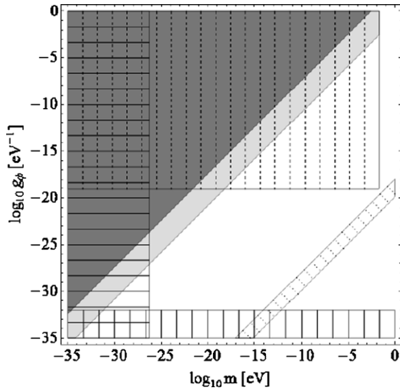
Figure 2. Plane (\log_{10} m [\text{eV}], \log_{10} g_\phi [\text{eV}^{-1}]) : region excluded by CAST (Andriamonje et al. 2007; white with dashed vertical lines), region where |\theta_{\text{CMB}}(\Omega_{\text{MAT}} = 0.3, m, g_\phi)| > 10^\circ obtained by the constant angle approximation in Finelli & Galaverni (2009) (light gray region), region where |\theta_{\text{HzRG}}(\Omega_{\text{MAT}} = 0.3, m, g_\phi)| > 5.0^\circ (dark gray with dashed vertical lines), (m, g_\phi) values expected in main QCD axion models (dotted slanted lines), region where the mass of the pseudo-scalar field is too small in order to explain dark matter ( m < 3H_{\text{eq}} ; white with horizontal lines), and region where PQ symmetry is broken at energies higher than Planck scale ( f_a > M_{\text{pl}} ; white with vertical lines).
