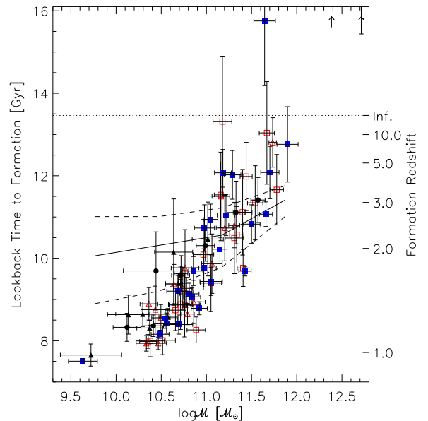
FIG. 3.— The formation epoch for the ETG shown in figure 1 (same symbols), evaluated as explained in the text. The two upward pointing arrows indicate that the two most massive cluster ETG are out of the figure (their ages amount to 16.4 and 23.4 Gyr). The continuous line shows the median model ages obtained by De Lucia et al. (2006) from a semianalytic model of hierarchical galaxy evolution, while the dashed lines are their upper and lower quartiles. More massive ETG form earlier in all environments, and the ages are not influenced by the environment.
